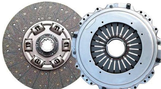
品名: 欧曼510PHC四级减震从动盘总成/压盘总成 Product Name: Auman 430 PHC driven disc assembly/Cover 规格: 430*240*10*52.5/430*240*475 Specification: 430*240*10*52.5/430*240*475 适配车型: 重汽汕德卡 福田欧曼 陕汽红岩 Fit models: Sinotruk Shande truck Auman Shanqi Red Rock
