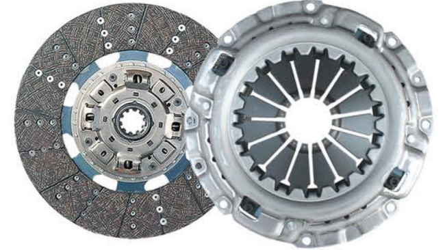
品名: 350欧马可压盘及从动盘总成 Product Name: 350 Aumark driven disc assembly 规格: 350*216*381/350*210*10*38.1 Specification: 350*216*381/350*210*10*38.1 适配车型: 福田欧马可 江淮奥铃 解放J6 Fit models: Aumark JACAoling FAWJ6
