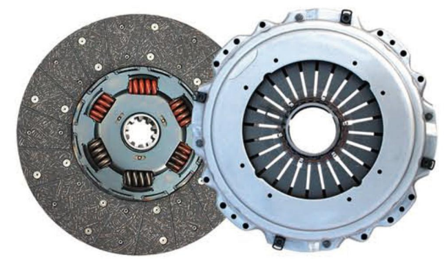
品名: 豪沃从动盘总成/压盘总成 Product Name: Pull the 430 driven disc assembly/Cover 规格: 430*260*10*52.5/430*240*475 Specification: 430*260*10*52.5/430*240*475 适配车型: 重汽豪沃 欧曼重卡 江淮格尔发 Fit models: Truck HOWO AUMAN JAC Gallop
