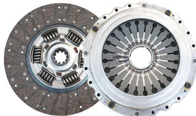
品名: 430伊顿四级减震从动盘总成/压盘总成 Product Name: Eaton 430 driven disc assembly/Cover 规格: 430*240*10*50.8/430*240*475 Specification: 430*240*10*50.8/430*240*475 适配车型: 美国伊顿、解放J6 Fit models: Eaton USA FAW J6
