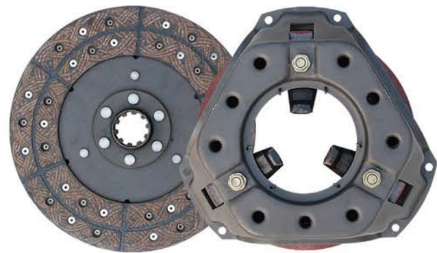
品名: NJ130从动盘总成/压盘总成 Product Name: NJ130 driven disc assembly/Cover 规格: 245*140*10*35.1/254*140*290 Specification: 254*140*10*35.1/254*140*290 适配车型: 福田轻卡 江淮 农用车 Fit models: Futian light truck jianghuai agricultural vehicle
