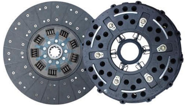
品名: 420从动盘总成/压盘总成 Product Name: Pull the 420 driven disc assembly/Cover 规格: 420*220*10*44.6/420*220*450 Specification: 420*220*10*44.6/420*220*450 适配车型: 潍柴 玉柴 道依茨 Fit models: Deutz Weichai Yuchai
