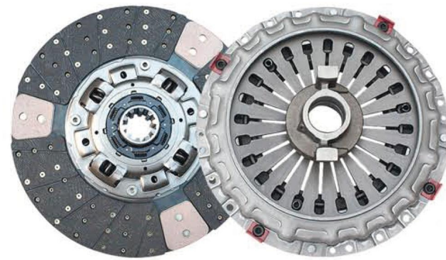
品名: 430五十铃从动盘总成/压盘总成 Product Name: Pull the 430 driven disc assembly/Cover 规格: 430*250*10*50.8/430*255*475 Specification: 430*260*10*52.5/430*255*475 适配车型: 五十铃6WF1 四桥水泥运输车 Fit models: ISUZU 6WF1 Four Bridge Cement Conveyor
