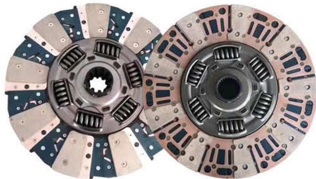
品名: 430伊顿四级减震从动盘总成/ Product Name: Pull the 430 driven disc assembly/Cover 规格: 430*240*10*50.8/24*50 Specification: 430*240*10*50.8/24*50 适配车型: 美国伊顿、东风天龙旗舰 Fit models: Eaton USA Dongfeng Tianlong flagship
