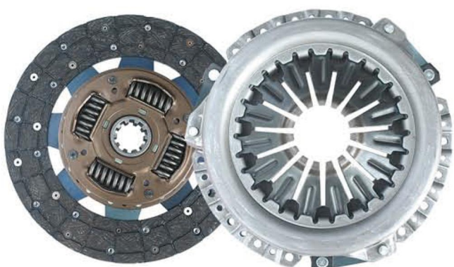
品名: 255欧马可压盘及从动盘总成 Product Name:255 Aumark driven disc assembly 规格: 255 *160*290/255*158*10*35 Specification:255 *160*290/255*158*10*35 适配车型: 福田康明斯欧马可 江淮奥铃 Fit models:Cummings Aumark JAC Aoling
