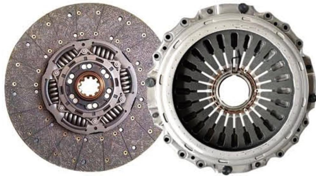
品名: 430LUK四级减震从动盘总成/压盘总成 Product Name: Pull the 430 LUK driven disc assembly/Cover 规格: 430*240*10*50.8/430*240*475 Specification: 430*240*10*50.8/430*240*475 适配车型: 伊顿、陕汽德龙、X3000 新M3000 Fit models: Eaton Shaanxi X3000 M3000
