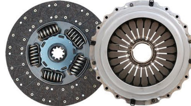
品名: 430大五簧四级减震从动盘总成/雷诺压盘总成 Product Name: Pull the 430 driven disc assembly/Cover 规格: 430*260*10*52.5/430*260*470 Specification: 430*260*10*52.5/430*260*470 适配车型: 伊顿、陕汽德龙、X3000 新M3000 Fit models: Eaton Shaanxi X3000 M3000
