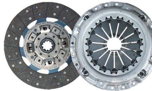
品名: 325五十铃压盘及从动盘总成 Product Name: 325 ISUZU driven disc assembly 规格: 325*195*368/325*190*14*35 Specification: 325*195*368/325*190*14*35 适配车型: 五十铃700P Fit models: ISUZU700P
