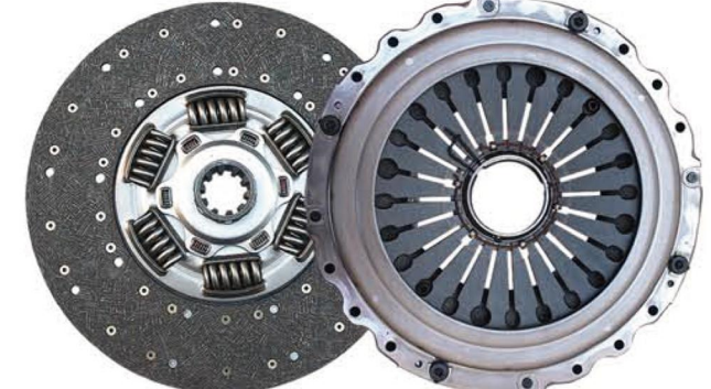
品名: 430法士特伊顿从动盘总成/伊顿压盘 Product Name: Pull the 430 driven disc assembly/Cover 规格: 430*240*10*50.8/430*260*475 Specification: 430*260*10*52.5/430*260*475 适配车型: 美国伊顿 解放JH6 Fit models: Eaton FAW JH6
