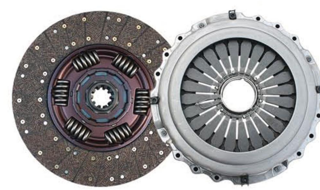
品名: 重汽T7从动盘总成/重汽压盘总成 Product Name: Pull the 430 driven disc assembly/Cover 规格: 430*260*10*52.5/430*240*475 Specification: 430*260*10*52.5/430*240*475 适配车型: 重汽T7 Fit models: Truck T7
