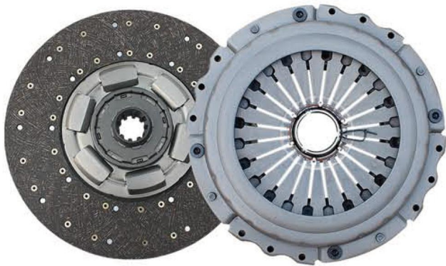
品名: 430大六从动盘总成/压盘总成 Product Name: Pull the 430 driven disc assembly/Cover 规格: 430*260*10*50.8/430*240*475 Specification: 430*260*10*50.8/430*240*475 适配车型: 重汽汕德卡 福田欧曼 陕汽红岩 玉柴 锡柴 潍柴 Fit models: Truck Shandeka AUMAN Yuchai Xichai Weichai Shaanxihongyan
