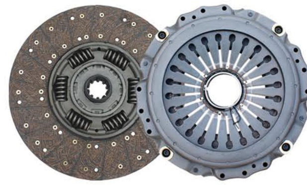
品名: 430三级减震从动盘总成/压盘总成 Product Name: Pull the 430 driven disc assembly/Cover 规格: 430*240*10*50.8/430*240*475 Specification: 430*260*10*50.8/430*240*475 适配车型: 金龙宇通客车 福田欧曼 陕汽红岩 玉柴 锡柴 潍柴 Fit models: Jinlong Yutong Bus Oman Yuchai Xichai Weichai Shaanxihongyan
